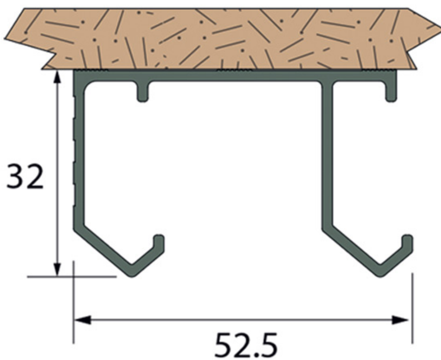
Rail 40 (1.94 - 3 m)
